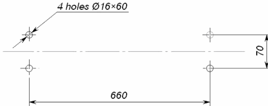
Figure 3 Installation holes for the MB-15R railing
