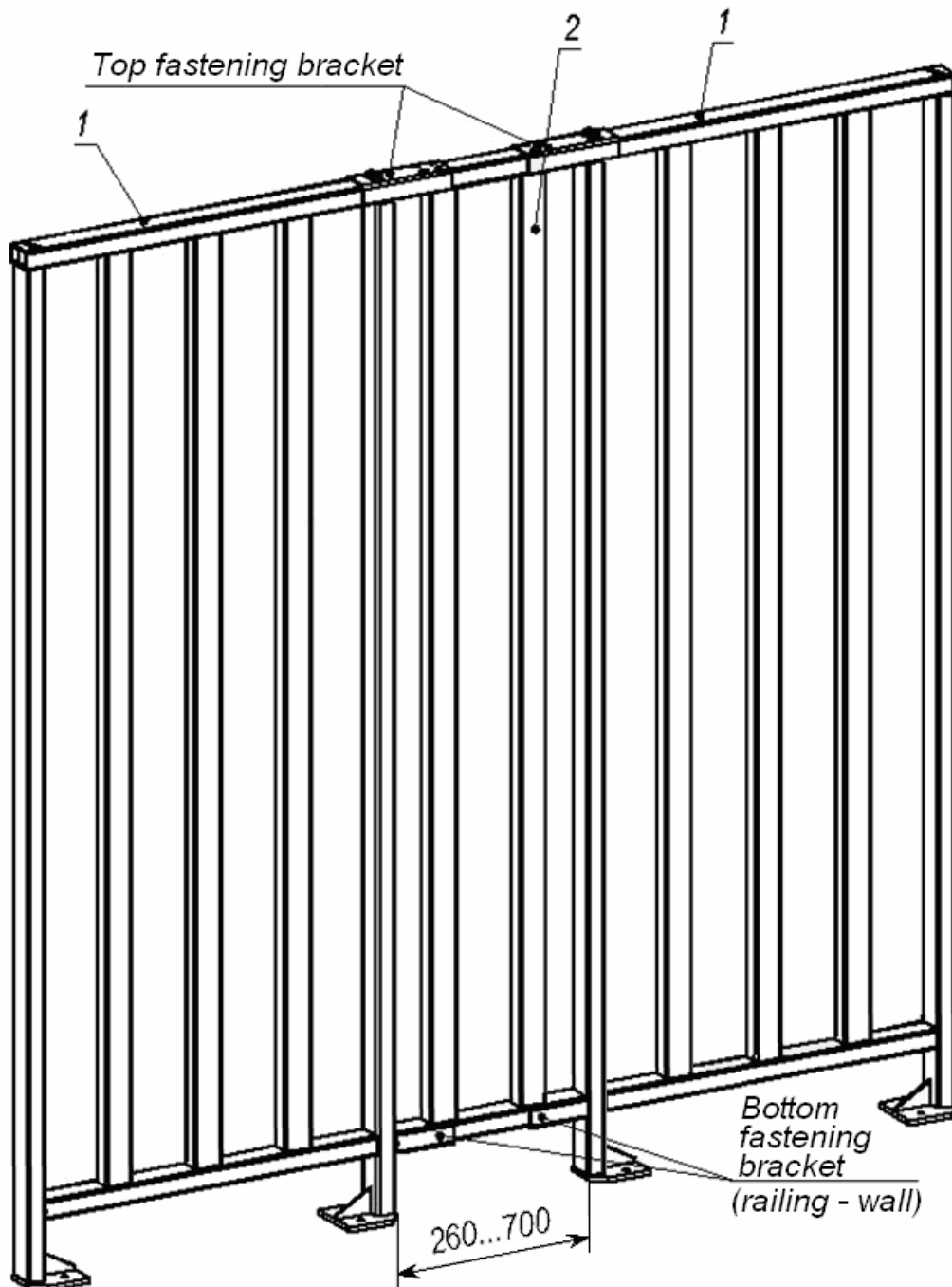
Figure 2 Sample design of the railings:
